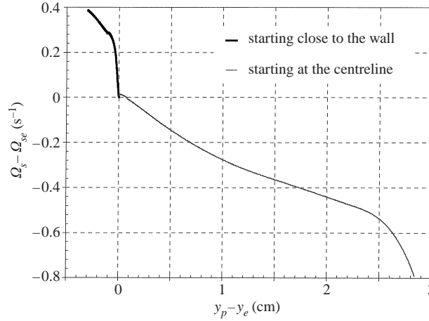
FIGURE 19. Analysis on the angular slip velocity discrepancy in the case of multiple equilibrium ( \rho_s/\rho_f = 1.01 , R = 20 ). Case (a), particle released close to the wall: ( y_p(t = 0) = 1.0 ). Case (b), particle released at the centreline: ( y_p(t = 0) = 6.0 ). For this data, the buoyancy force intersects the lift force at three points, and two of them yield stable solutions (figure 5). For case (a), the particle travels from a position close to the wall to the equilibrium height closer to the wall y_e = 1.323 cm, whereas for case (b), the particle travels from the centreline to the equilibrium height far from the wall y_e = 3.165 cm. The discrepancy changes sign at the equilibrium y_p = y_e where the lift balances the buoyant weight.
