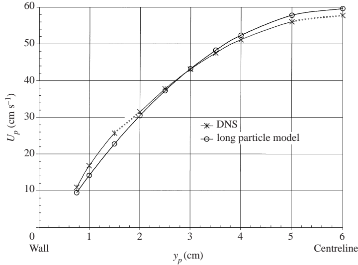
FIGURE 24. Particle velocity vs. particle position.
