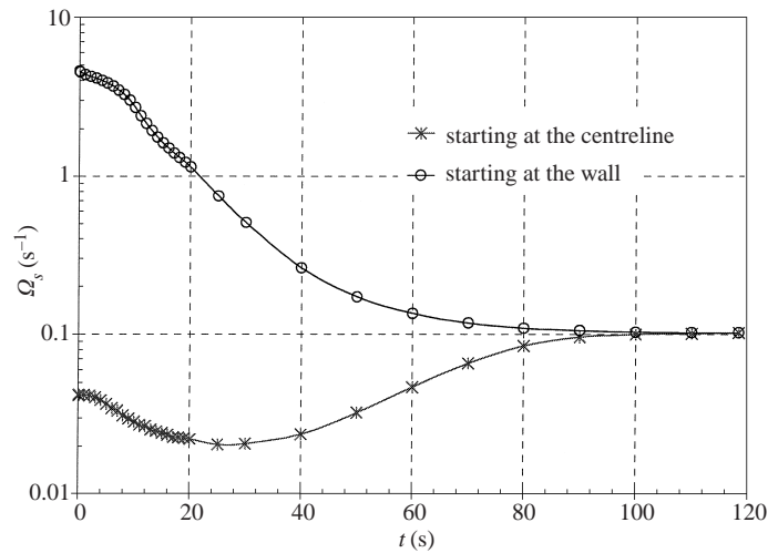
FIGURE 10. Evolution of the angular slip velocity of a neutrally buoyant particle at R = 10 to equilibrium (see figure 8). The angular slip velocity function evolves without crossing the equilibrium value. When the angular slip velocity is below the equilibrium value, the particle moves downward. When the angular slip velocity is above the equilibrium value, the particle moves upward.
